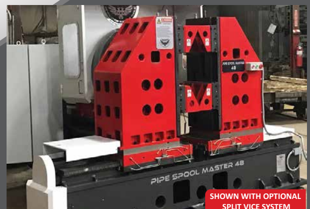
Heavy Duty Pipe Vices
